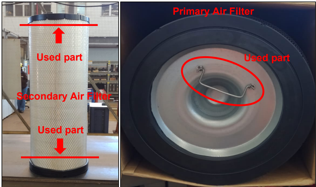
Picture 2: Air Filter, Primary and Secondary.
