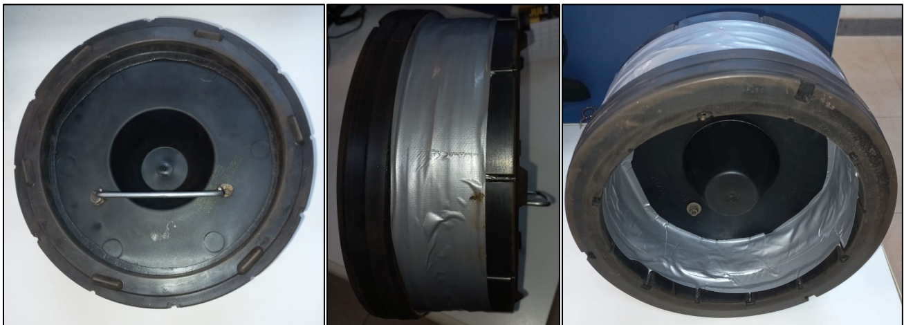
Picture 1: Tool to isolate air intake lines for pre-cleaner washing process.
